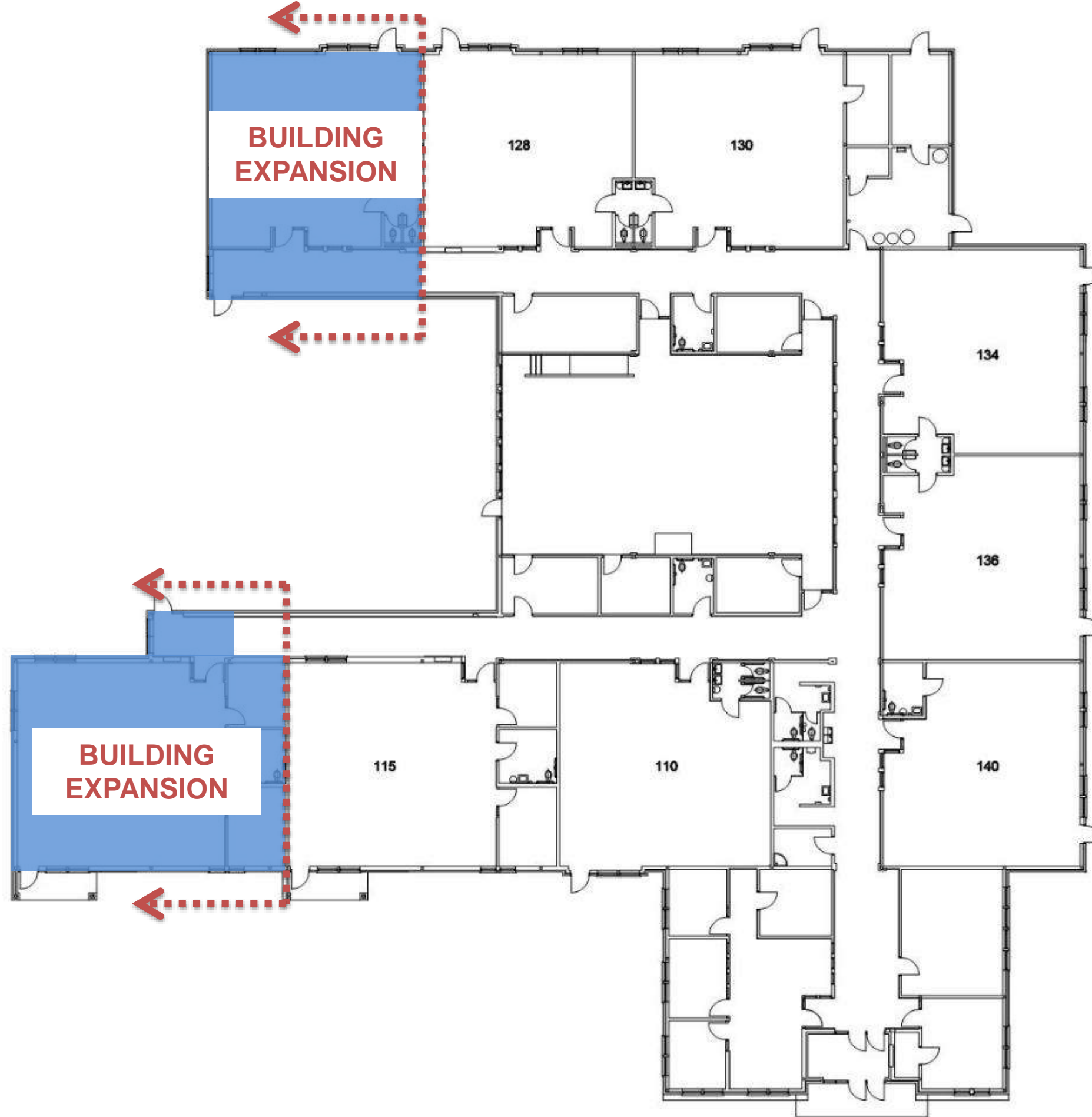
EARLY CHILDHOOD CENTER – preliminary floor plan expansion
